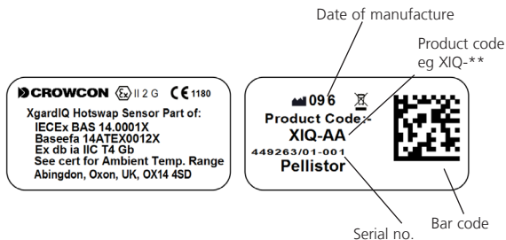
Diagram 6: Sensor module labels
