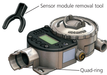
Diagram 19: Quad-ring location
